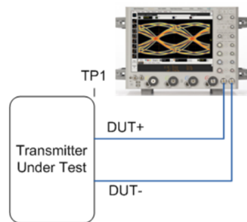
Figure 6 Probing for REFCLK Measurements
